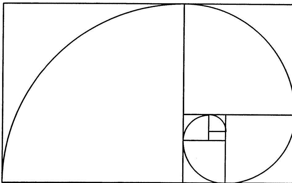
A visual presentation of the first six golden rectangles from the sequence of the rectangles represented by the table and the spiral curve associated with them.
